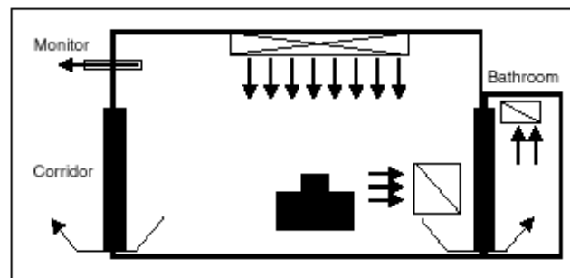
FIGURE 1. Example of positive-pressure room control for protection from airborne environmental microbes*†
